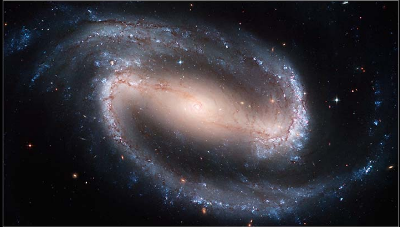
Barred Spiral Galaxy NGC 1300
